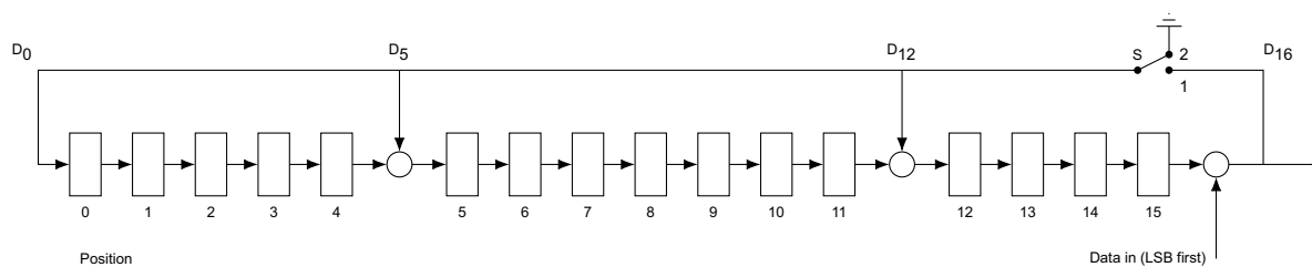
Figure 2.1: LFSR circuit generating the CRC
